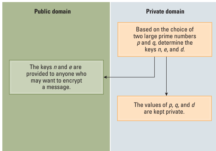
Figure 12.14 Establishing an RSA public-key encryption system
