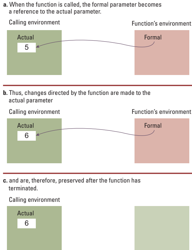
Figure 6.11 Executing the function Demo and passing parameters by reference
