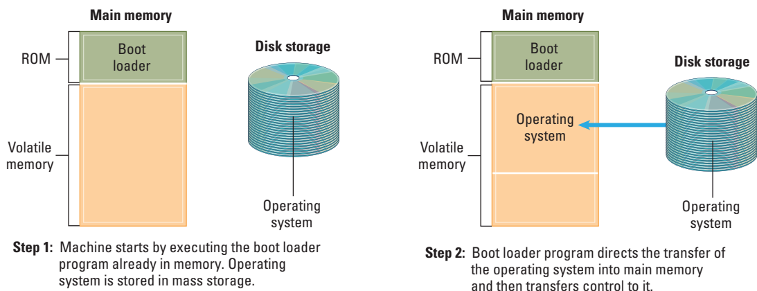
Figure 3.5 The booting process
