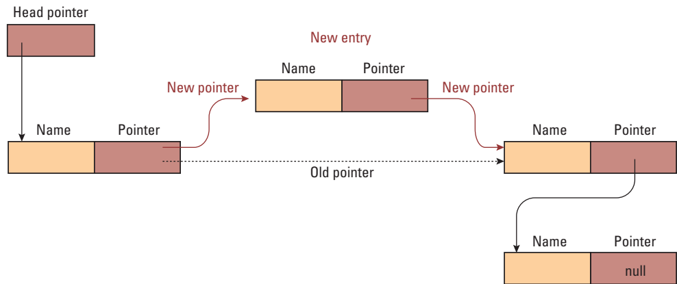
Figure 8.11 Inserting an entry into a linked list
