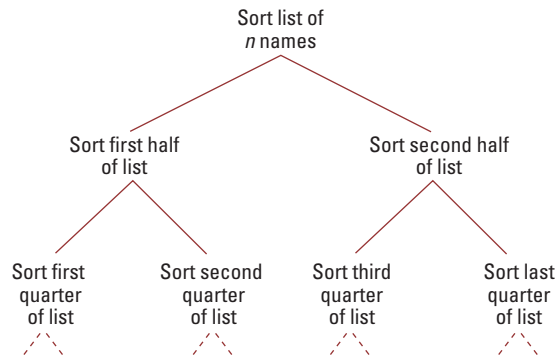
Figure 12.10 The hierarchy of problems generated by the merge sort algorithm
