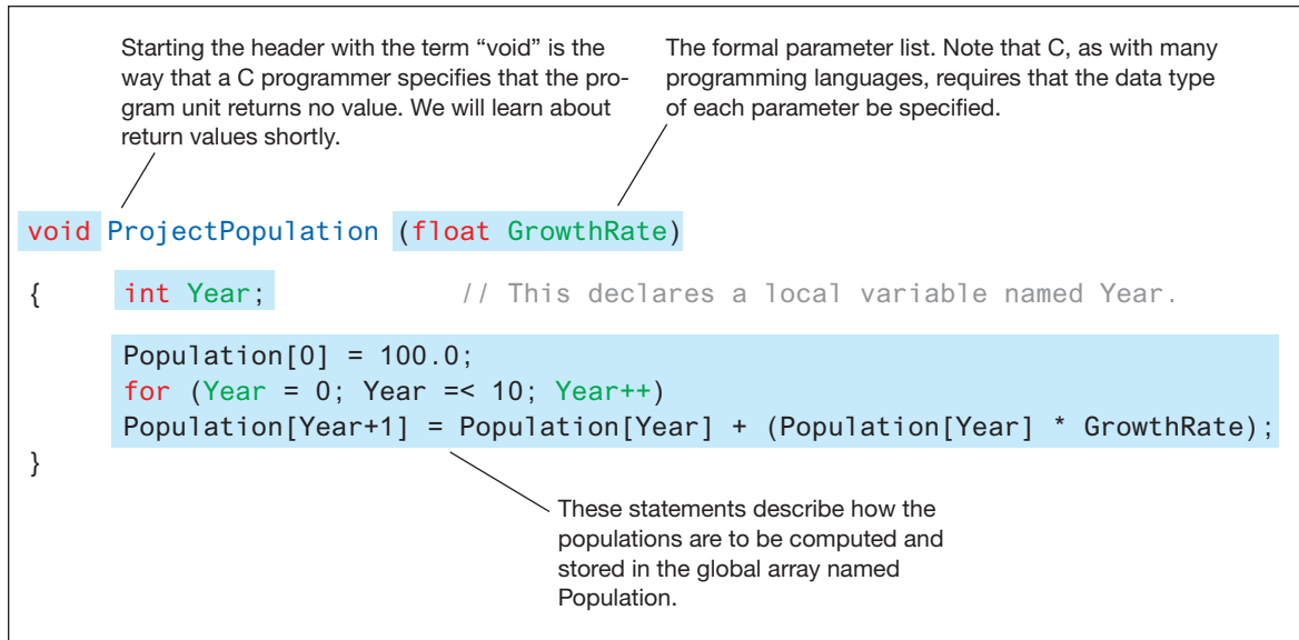
Figure 6.9 The function ProjectPopulation written in the programming language C
