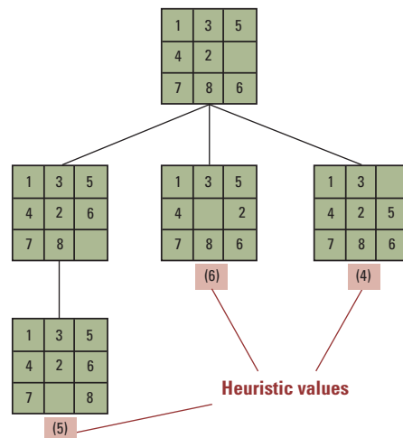
Figure 11.12 The search tree after two passes
