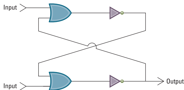
Figure 1.5 Another way of constructing a flip-flop
