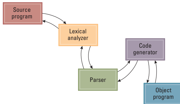
Figure 6.18 An object-oriented approach to the translation process
