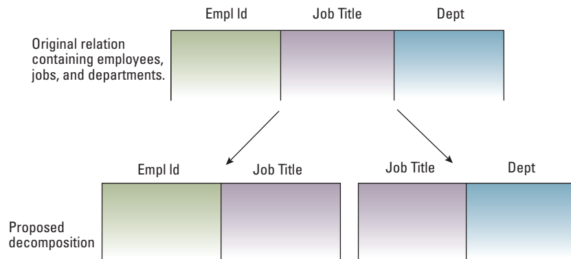
Figure 9.7 A relation and a proposed decomposition
