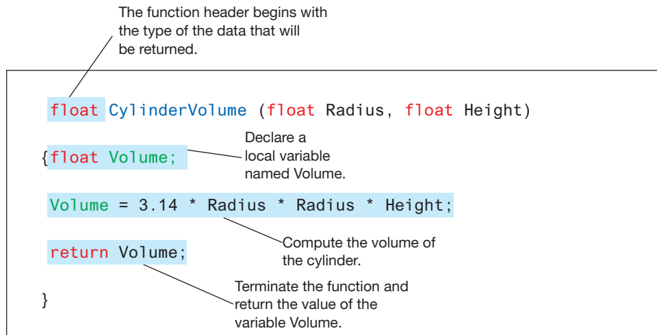
Figure 6.12 The fruitful function CylinderVolume written in the programming language C
