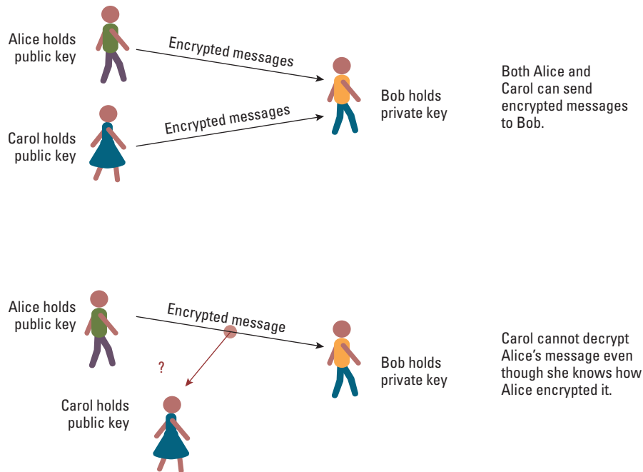
Figure 4.16 Public key encryption
