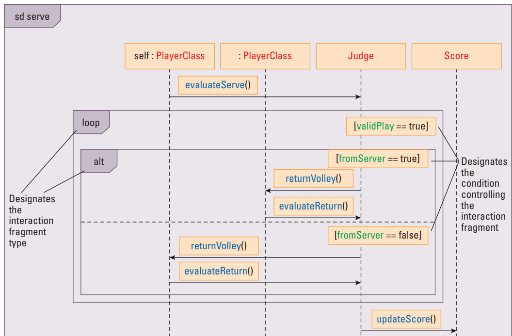
Figure 7.13 A sequence diagram depicting a generic volley
