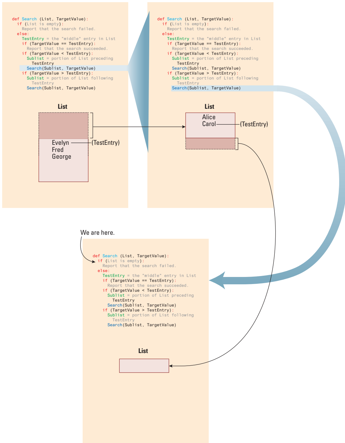
Figure 5.17 Second Recursive Search, Second Snapshot
