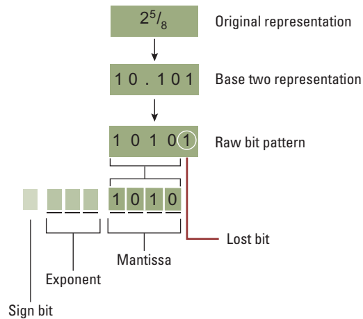
Figure 1.25 Encoding the value 2^5/8
