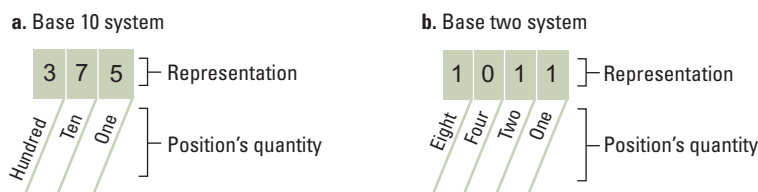
Figure 1.13 The base ten and binary systems
