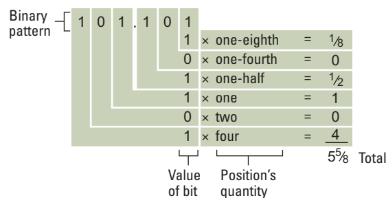
Figure 1.18 Decoding the binary representation 101.101
