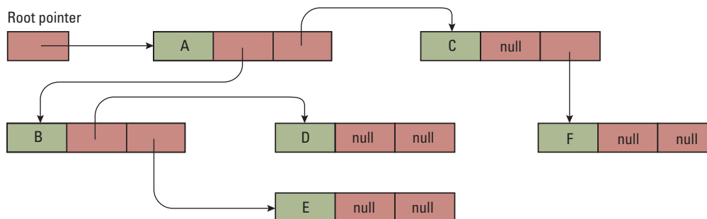
Figure 8.16 The conceptual and actual organization of a binary tree using a linked storage system
