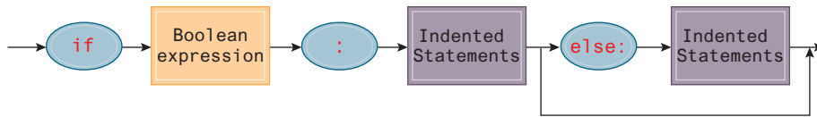
Figure 6.14 A syntax diagram of Python's if-else statement
