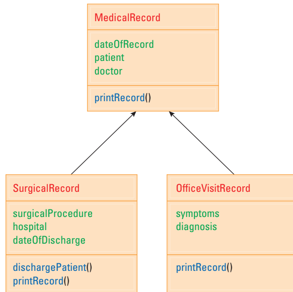
Figure 7.12 A class diagram depicting generalizations
