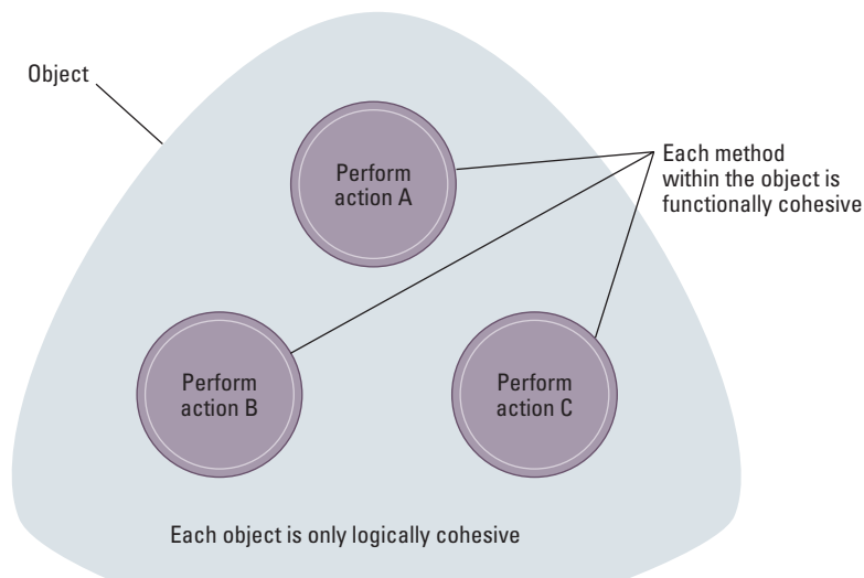
Figure 7.7 Logical and functional cohesion within an object
