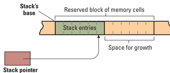
Figure 8.12 A stack in memory
