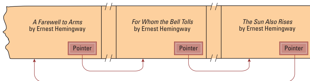
Figure 8.4 Novels arranged by title but linked according to authorship
