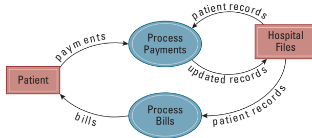
Figure 7.8 A simple dataflow diagram
