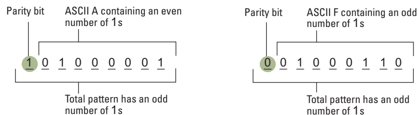
Figure 1.26 The ASCII codes for the letters A and F adjusted for odd parity
