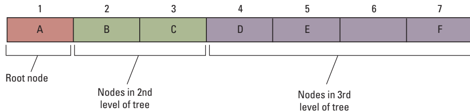
Figure 8.17 A tree stored without pointers
