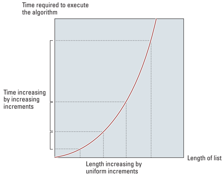
Figure 5.19 Graph of the worst-case analysis of the insertion sort algorithm
