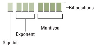
Figure 1.24 Floating-point notation components
