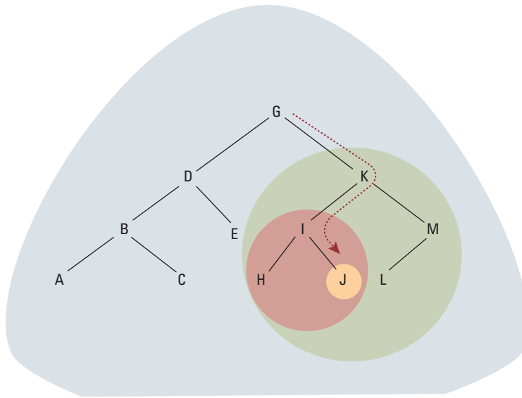
Figure 8.22 The successively smaller trees considered by the function in Figure 8.21 when searching for the letter J
