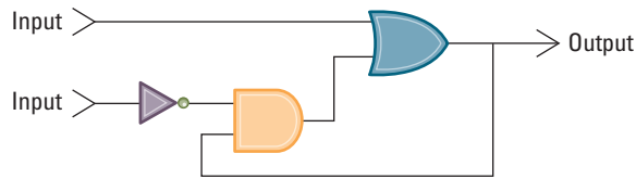
Figure 1.3 A simple flip-flop circuit
