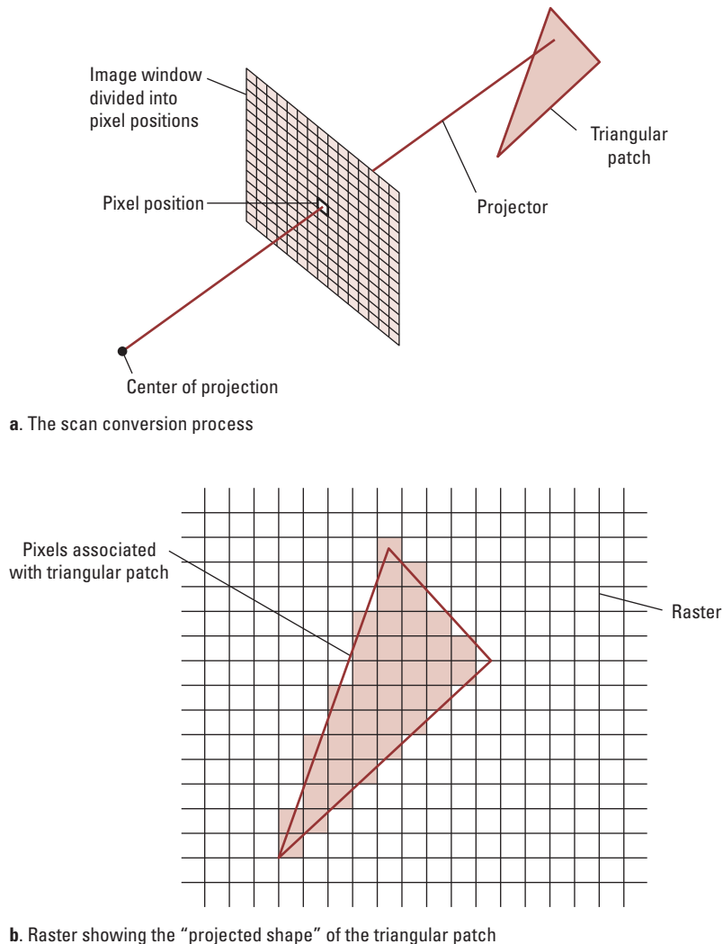
Figure 10.9 The scan conversion of a triangular patch
