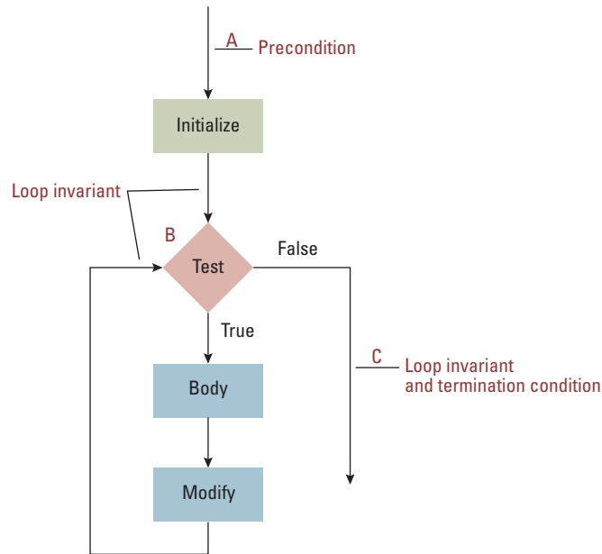
Figure 5.23 The assertions associated with a typical while structure
