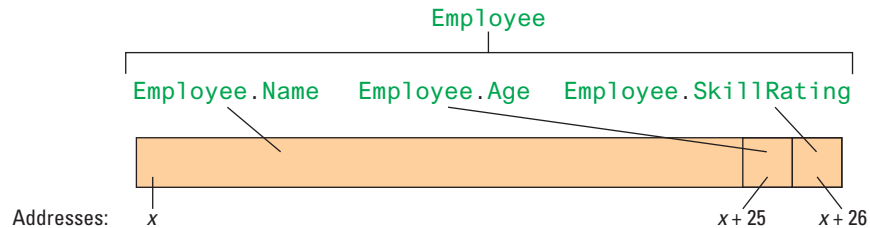
a. Aggregate stored in a contiguous block
