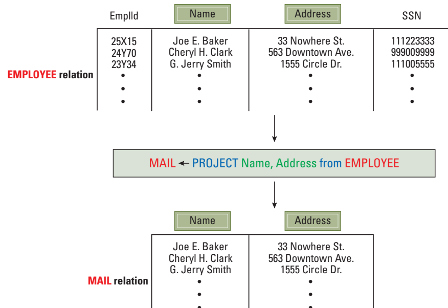
Figure 9.9 The PROJECT operation
