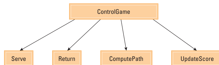
Figure 7.3 A simple structure chart
