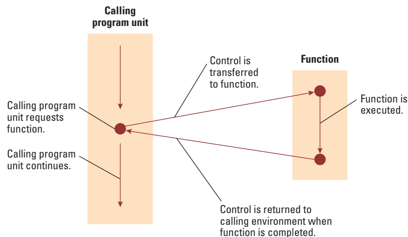
Figure 6.8 The flow of control involving a function
