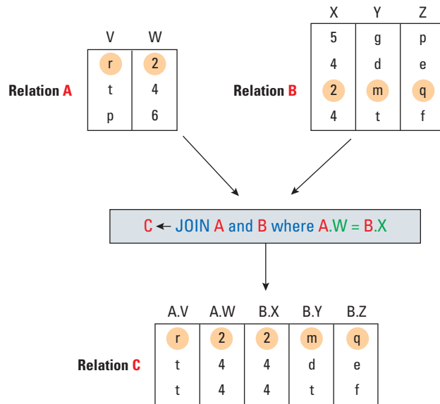
Figure 9.10 The JOIN operation
