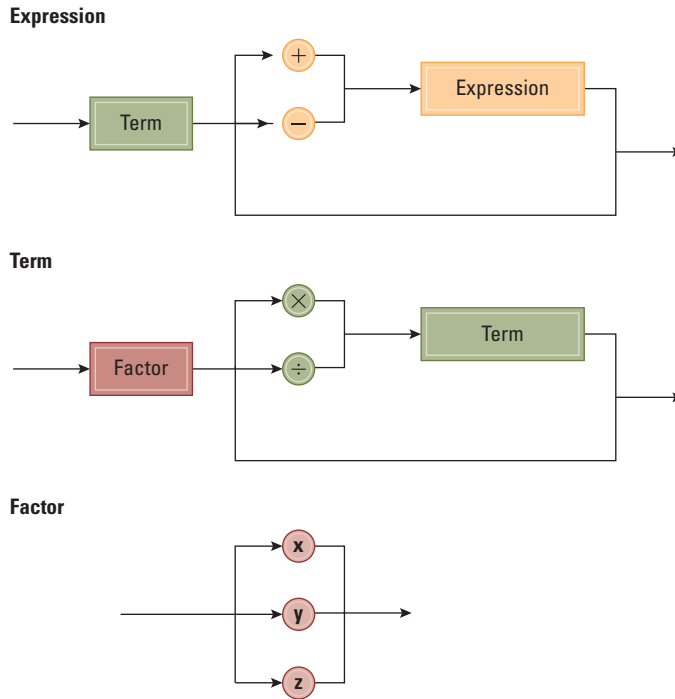
Figure 6.15 Syntax diagrams describing the structure of a simple algebraic expression
