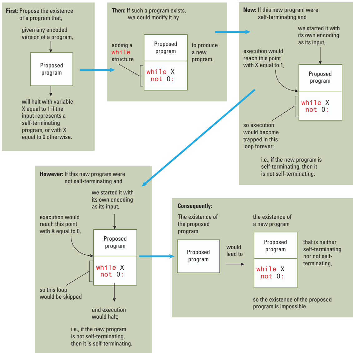
Figure 12.7 Proving the unsolvability of the halting program
