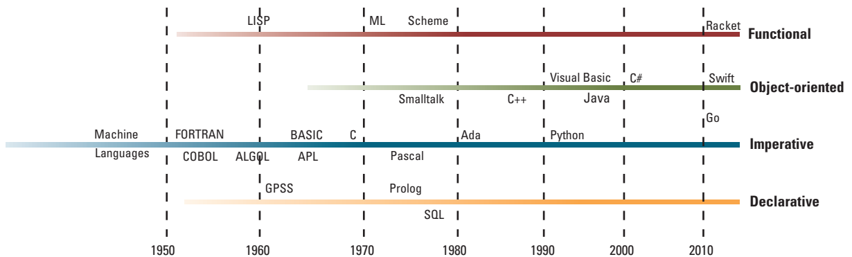
Figure 6.2 The evolution of programming paradigms
