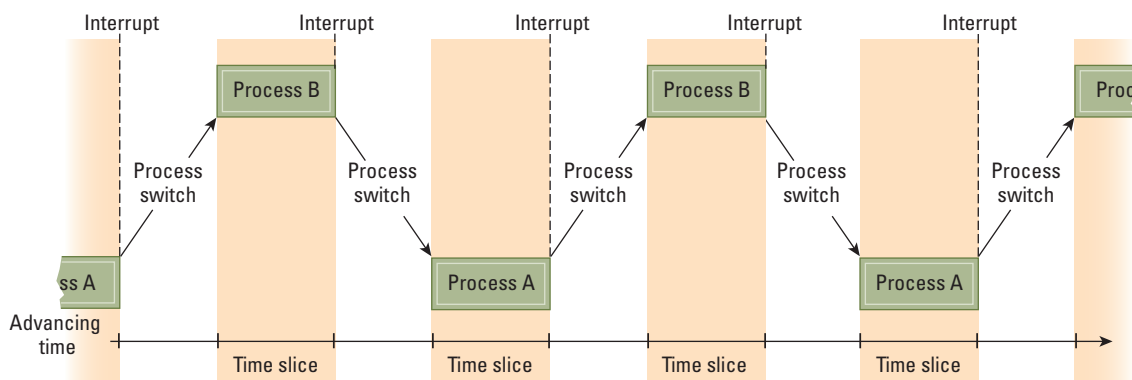
Figure 3.6 Multiprogramming between process A and process B
