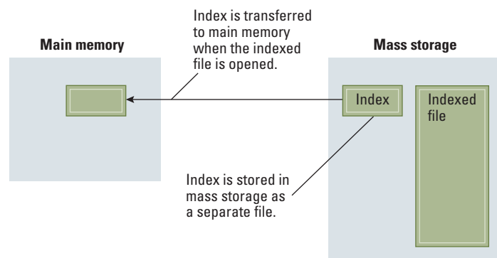
Figure 9.17 Opening an indexed file
