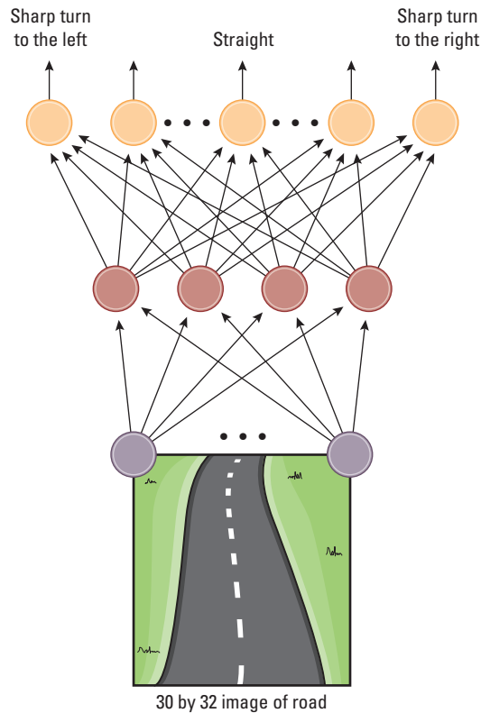
Figure 11.19 The structure of ALVINN (Autonomous Land Vehicle in a Neural Net). Based on the structure of ALVINN by Dean A. Pomerleau.
