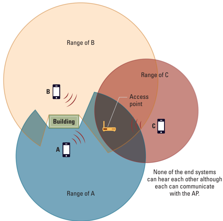
Figure 4.3 The hidden terminal problem
