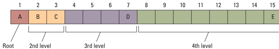
Figure 8.18 A sparse, unbalanced tree shown in its conceptual form and as it would be stored without pointers
