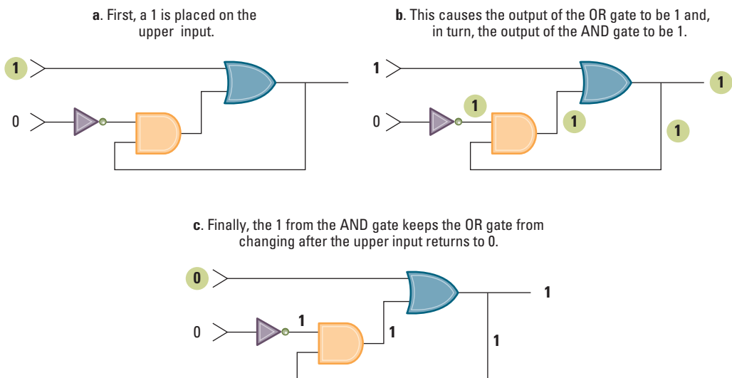
Figure 1.4 Setting the output of a flip-flop to 1
