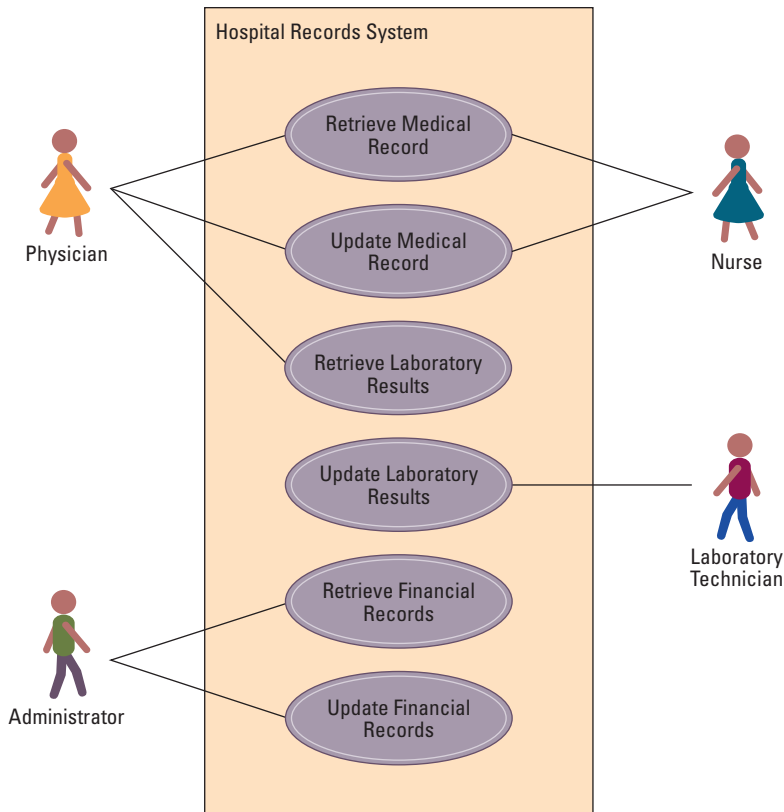
Figure 7.9 A simple use case diagram
