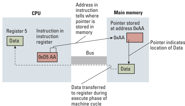
Figure 8.28 Our first attempt at expanding the Vole machine language in Appendix C to take advantage of pointers
