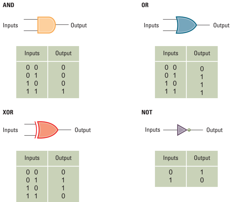
Figure 1.2 A pictorial representation of AND, OR, XOR, and NOT gates as well as their input and output values
