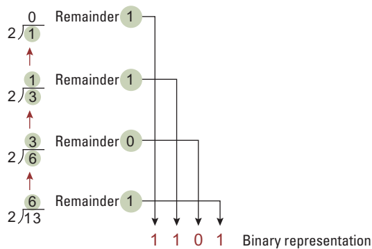
Figure 1.16 Applying the algorithm in Figure 1.15 to obtain the binary representation of thirteen
