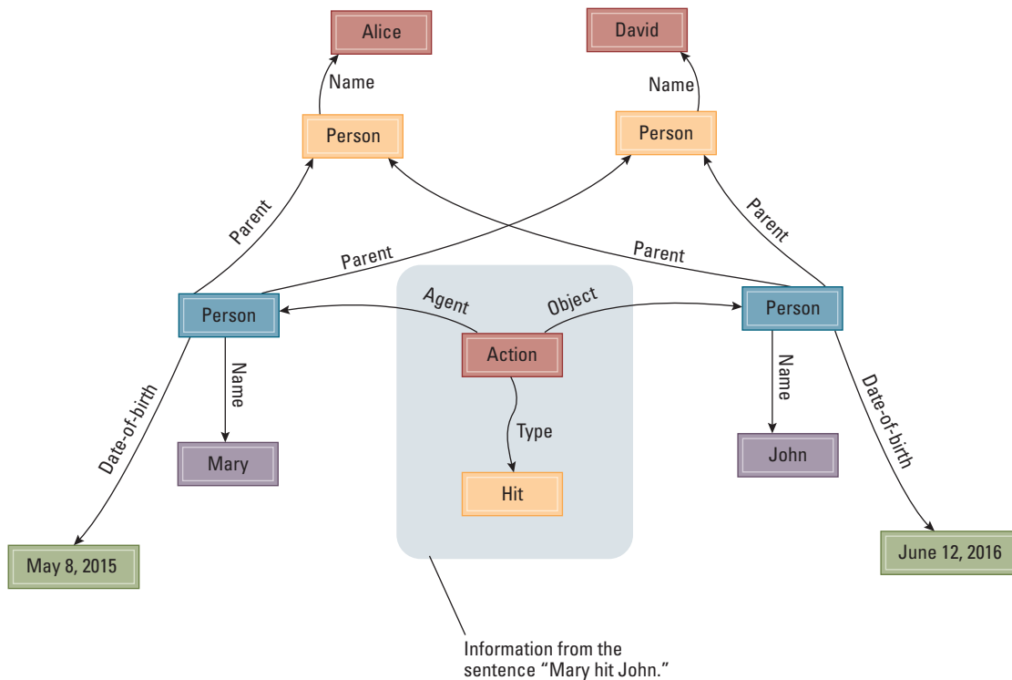
Figure 11.3 A semantic net
