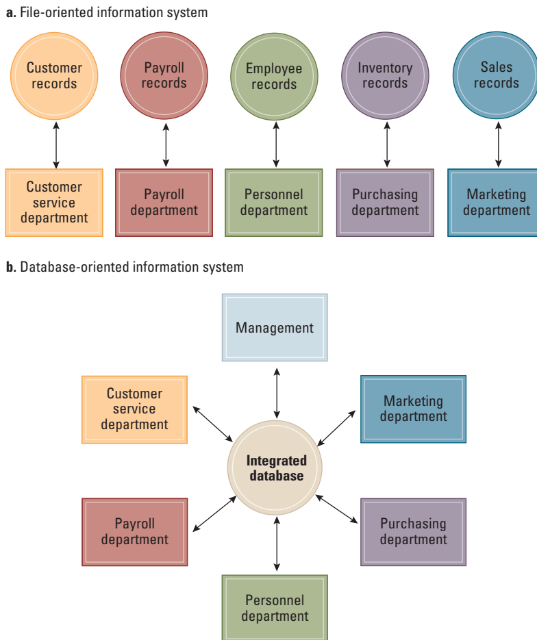
Figure 9.1 A file versus a database organization
