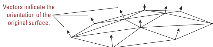
Figure 10.11 A conceptual view of a polygonal mesh with normal vectors at its vertices
