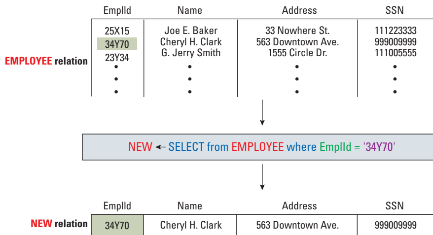
Figure 9.8 The SELECT operation
