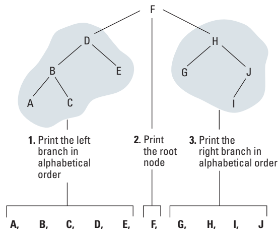
Figure 8.23 Printing a search tree in alphabetical order
