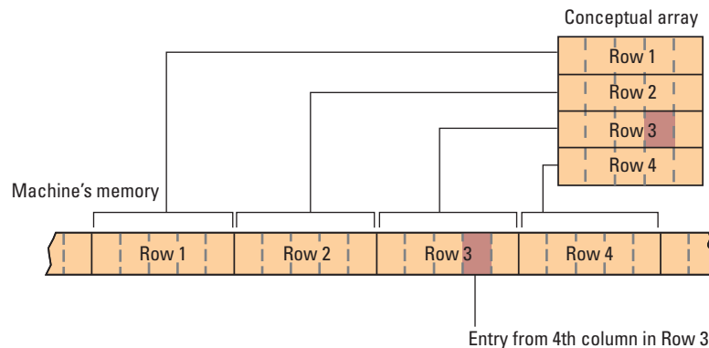
Figure 8.6 A two-dimensional array with four rows and five columns stored in row major order
