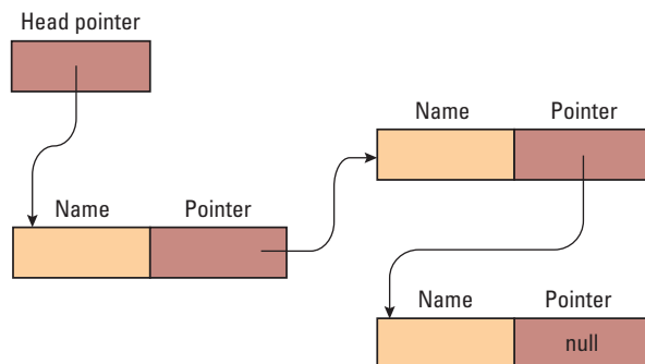
Figure 8.9 The structure of a linked list
