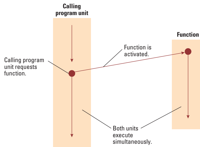
Figure 6.23 Spawning threads
