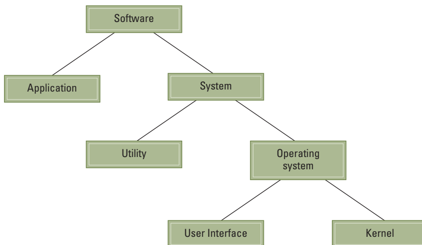
Figure 3.3 Software classification
