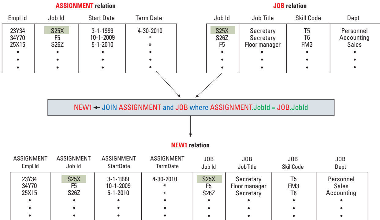
Figure 9.12 An application of the JOIN operation
