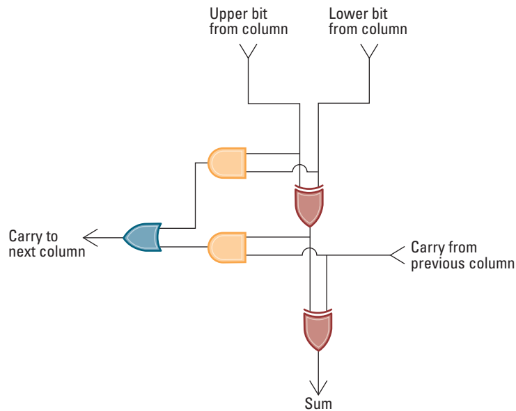
Figure B.2 A circuit to add a single column in a multiple-column addition problem
