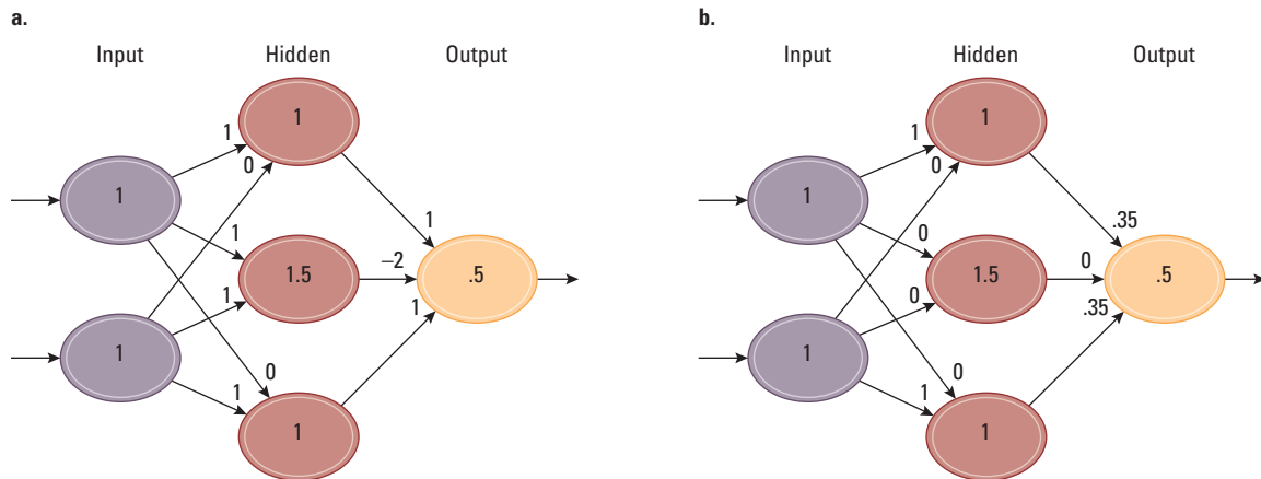
Figure 11.18 A neural network with two different programs
