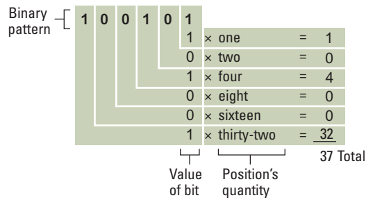
Figure 1.14 Decoding the binary representation 100101
