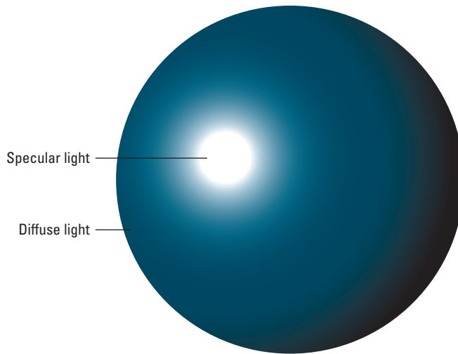
Figure 10.6 Specular versus diffuse light
