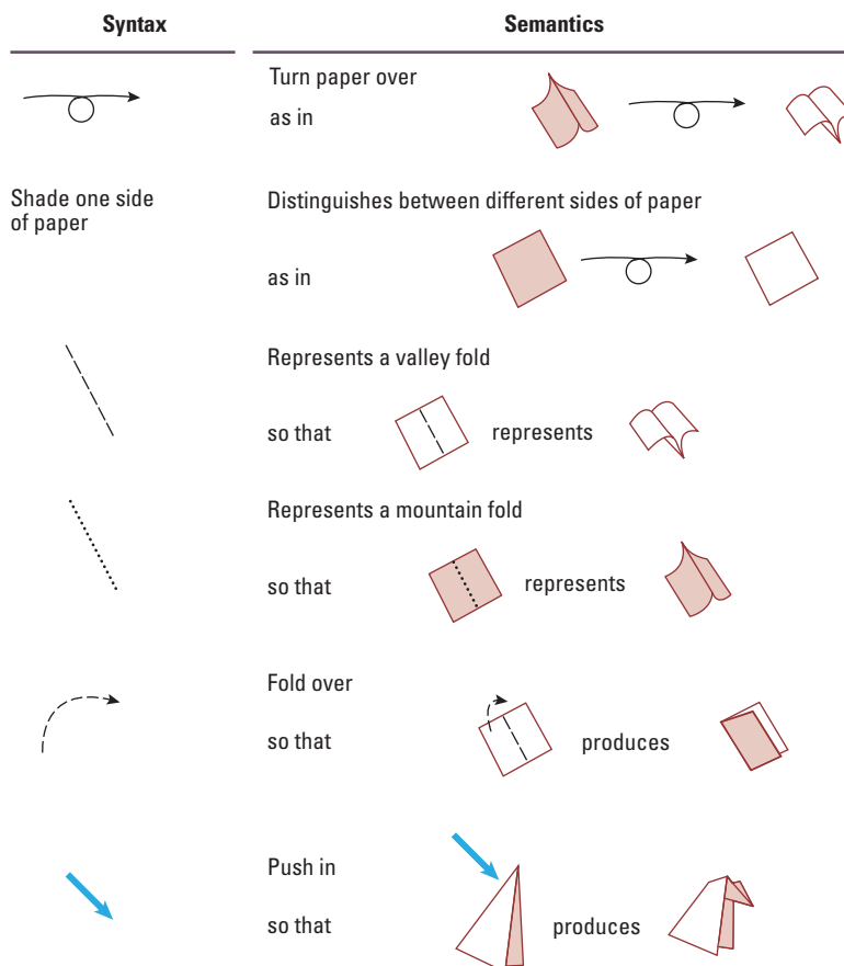
Figure 5.3 Origami primitives
