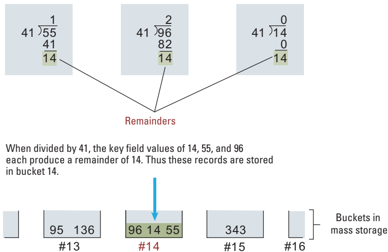
Figure 9.19 The rudiments of a hashing system
