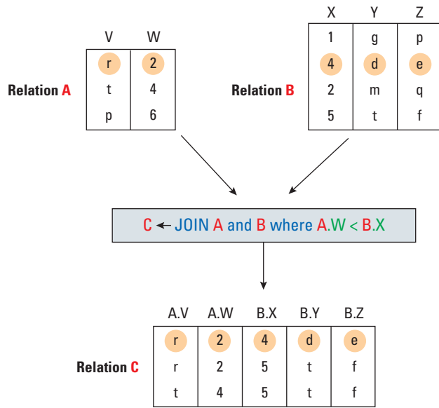
Figure 9.11 Another example of the JOIN operation
