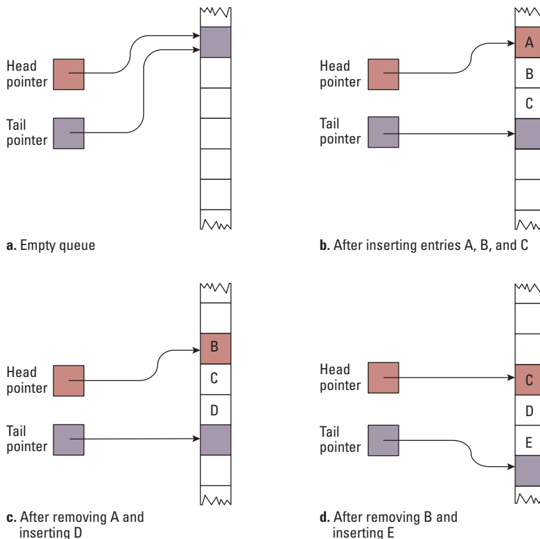
Figure 8.13 A queue implementation with head and tail pointers. Note how the queue crawls through memory as entries are inserted and removed.
