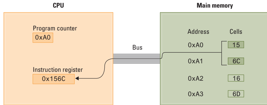
a. At the beginning of the fetch step, the instruction starting at address 0xA0 is retrieved from memory and placed in the instruction register.
