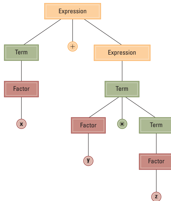
Figure 6.16 The parse tree for the string x + y \times z based on the syntax diagrams in Figure 6.15
