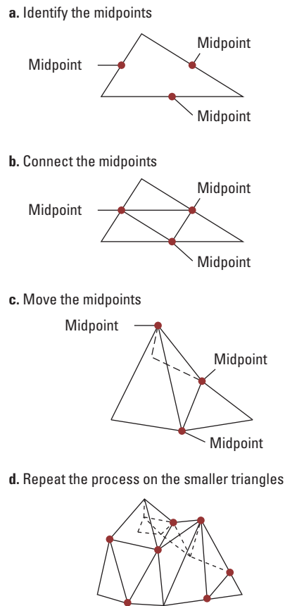
Figure 10.4 Growing a polygonal mesh for a mountain range
