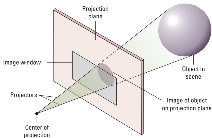
Figure 10.1 The 3D graphics paradigm
