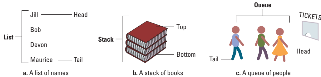
Figure 8.1 Lists, stacks, and queues
