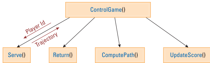
Figure 7.6 A structure chart including data coupling
