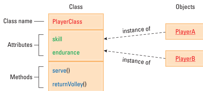
Figure 7.4 The structure of PlayerClass and its instances
