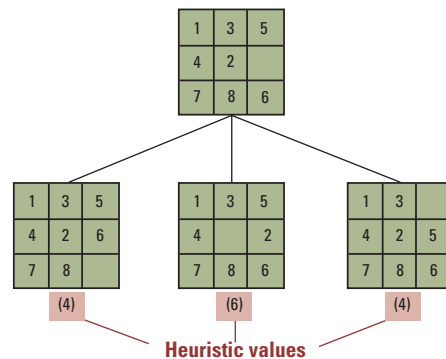
Figure 11.11 The beginnings of our heuristic search
