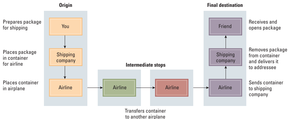
Figure 4.12 Package-shipping example
