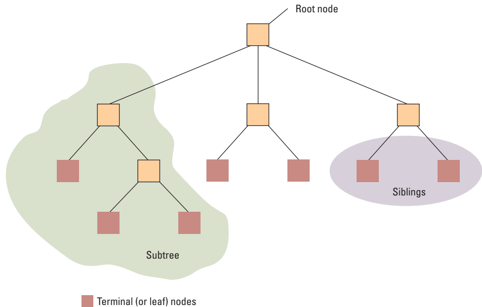
Figure 8.3 Tree terminology
