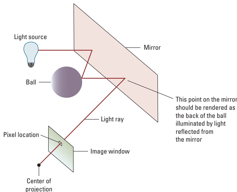
Figure 10.13 Ray tracing
