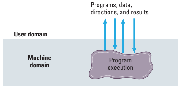
Figure 3.2 Interactive processing
