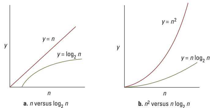
Figure 12.11 Graphs of the mathematical expressions n , \log_2 n , n \log_2 n , and n^2
