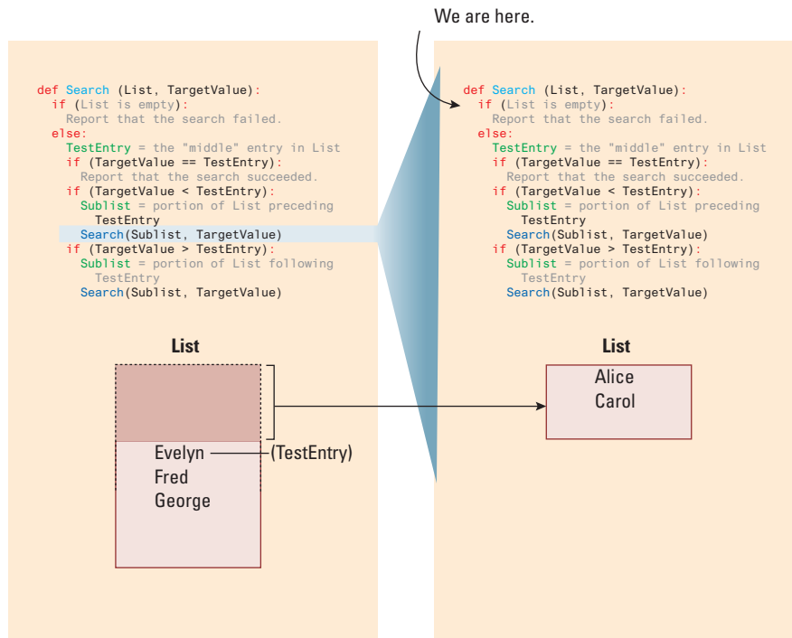
Figure 5.16 Second Recursive Search, First Snapshot
