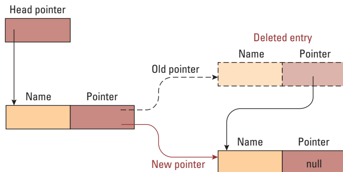
Figure 8.10 Deleting an entry from a linked list
