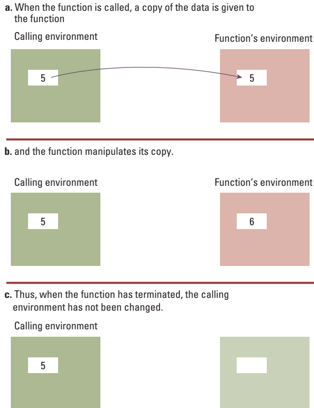
Figure 6.10 Executing the function Demo and passing parameters by value
