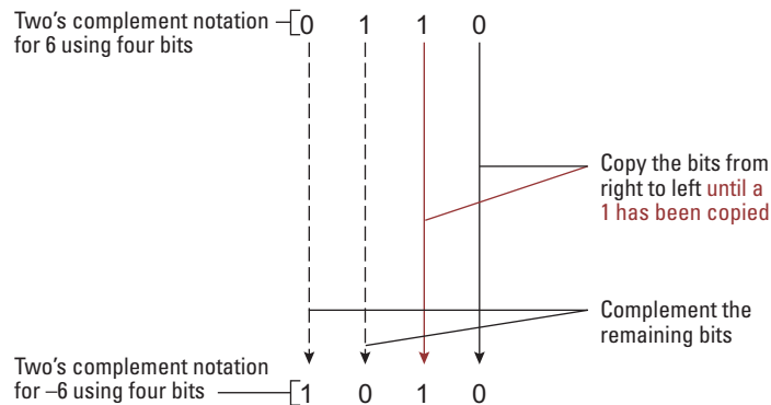
Figure 1.20 Encoding the value -6 in two's complement notation using 4 bits
